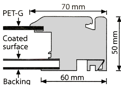
70 mm profile - 50 mm depth
