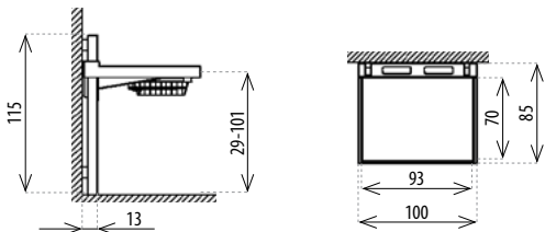
BSR105: Wall-mounted changing table
