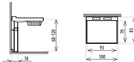
BSR121: Wall-mounted changing table, single column
