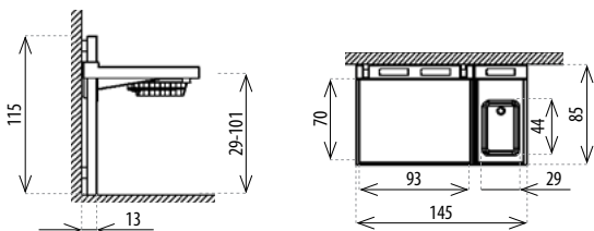
BSR107: Wall-mounted changing table with sink
