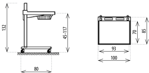
BSR119: Free-standing changing table with wheels
